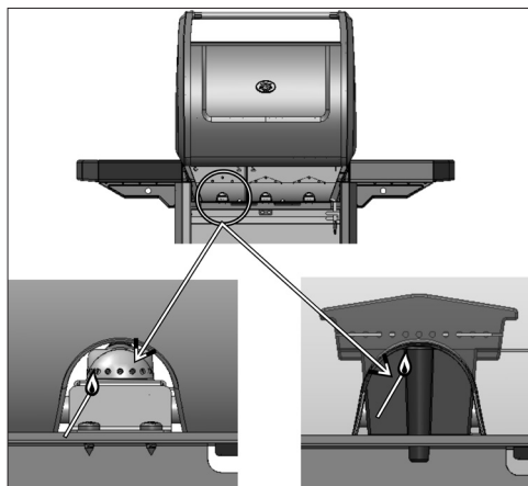
stainless steel burner
